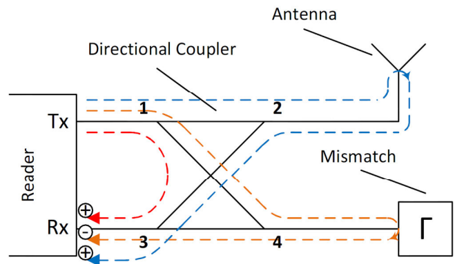
Fig. 2. Principle of the mismatched coupler
