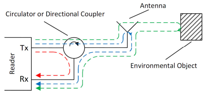
Fig. 1. Tx to Rx carrier leakage paths
