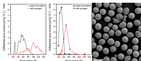
Fig. 3 Pore size distribution of sintered zirconia particles formed by the vibrational dispenser. left: data analyzed with the DFT-method; middle: data analyzed with the BJH method; right: SEM image, scale bar 100 µm.
