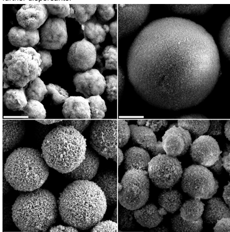
Fig. 4 Sintered particles formed by the PICA method. The scale bars represent 2 µm. top left: zirconia; top right: alumina; bottom left: titania; bottom right: ceria.
