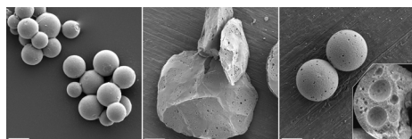
Fig. 1 SEM images of sintered zirconia particles produced by batchwise emulsification under different conditions. The scale bars correspond to 10 µm. The inset on the rightmost image represents a cross section of a particle.
