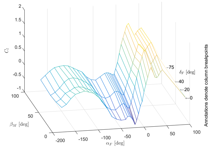
Fig. 2 XV-15 experimental data of the aerodynamic lift coefficient ( C_{LW} ) of the wing as a function of the mast tilt-angle ( \beta_M ), flap deflection ( \delta_F ) and angle of attack of the aircraft ( \alpha_F )
