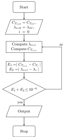
Fig. 1 Flow-chart of the Inflow-Thrust solution algorithm
