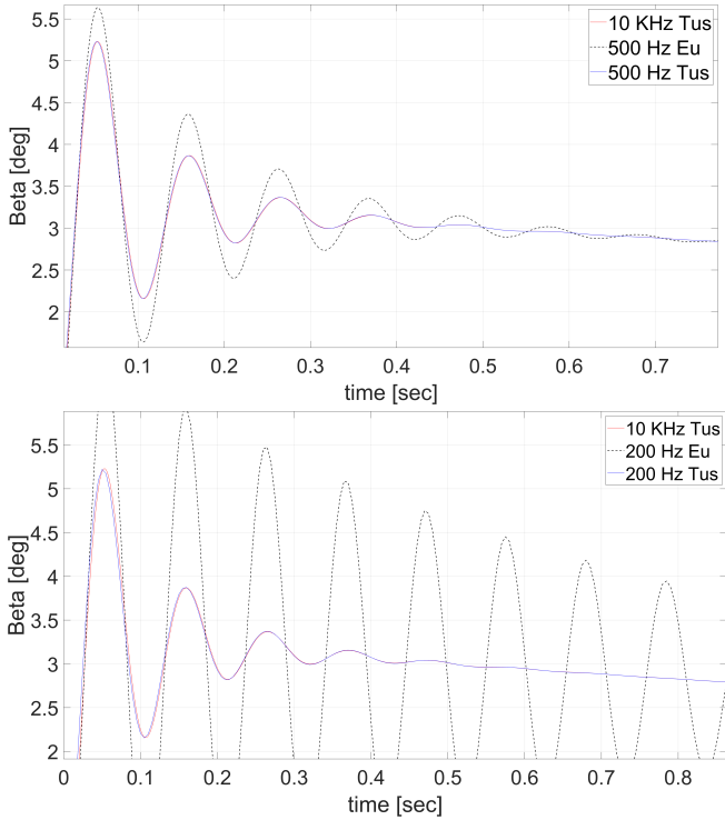
Fig. 10 Comparison between different sampling frequencies for Euler Integrators and the reference Tustin integrator (2 of 2)
