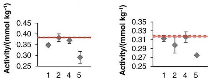
Fig. 10. Selected results of an interlaboratory comparison based on measurements of ion activities of Mg^{2+} and Ca^{2+} ions. Reference values are displayed in red color, activity values measured by ZHAW are depicted in column 4.
