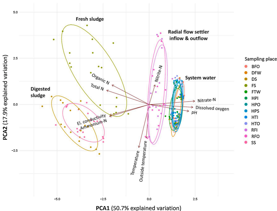
Fig. 3. Principal component analysis (PCA) with 95 % confidence ellipses of measured abiotic parameters and different nitrogen forms in the different compartments (FTW, fish tank water; DFW, drum filter outflow water; BFO, biofilter outflow water; HPI, inflow into hydroponic part of the system; HPS, sump water; HTI, hydroponic table inflow; HTO, hydroponic table outflow; HPO, outflow from hydroponic part of the system; RFI, radial flow settler inflow; RFO, radial flow settler outflow; FS, settled fresh sludge; DS, digested sludge; SS, supernatant of digested sludge returned back to the system) of the aquaponic system, measured six times during the experiment, explaining 68.6 % of data variance ( n > 14 ).
