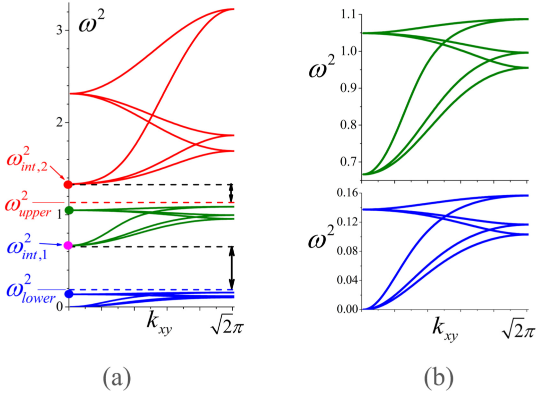
Fig. 6. (a) Cross-sections of frequency surfaces ( k_x = k_y = k_{xy}/\sqrt{2}, k_z = 0 ), taking into account the internal structure of the lattice nodes. \Omega^2 = 1.5, \alpha = 2, \beta = 1 , and \gamma = 2 . (b) A more detailed representation of the blue and olive dependencies given in part (a). (For interpretation of the references to colour in this figure legend, the reader is referred to the web version of this article.)
