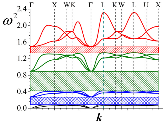
Fig. 15. The manifestation of an additional core inside the lattice node for the system shown in Fig. 14 ( \Omega_e^2 = 1.5, \alpha = 2, \beta = 1, \gamma = 2, \alpha' = 2, and \beta' = 0.5 ).
