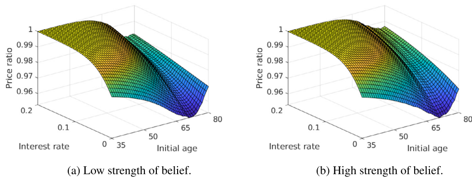
Fig. 10. Ratio between the annuity values of the joint and independent survival models using the B-RUP with different strengths of belief ((a) and (b)).
