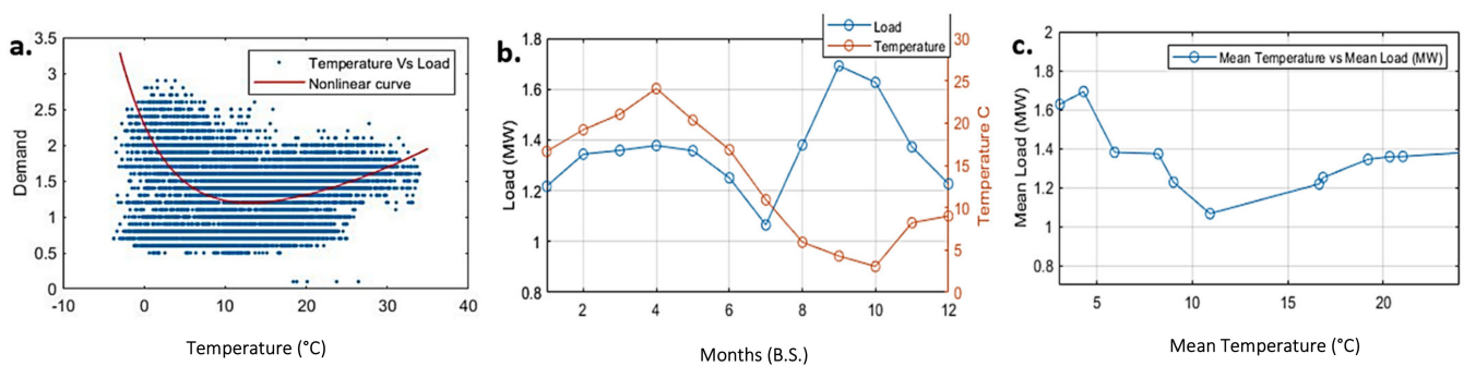
Figure 5. (a) Joint plot of the electric load vs. temperature. (b) Monthly mean plot of the electric load and temperature. (c) Mean plot of the temperature vs. electric load.
