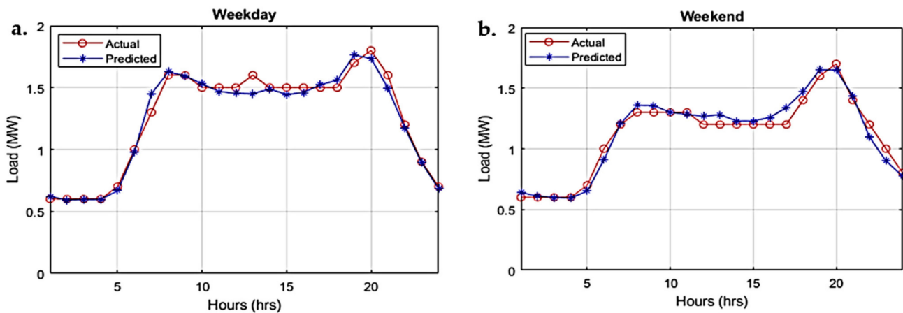
Figure 12. Actual vs. predicted forecasts achieved by the ANN models with (a) a double-layer 16 \times 16 node structure and (b) a single-layer 8 node structure.
