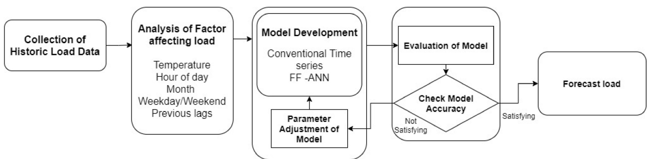
Figure 8. Forecasting methodology.
