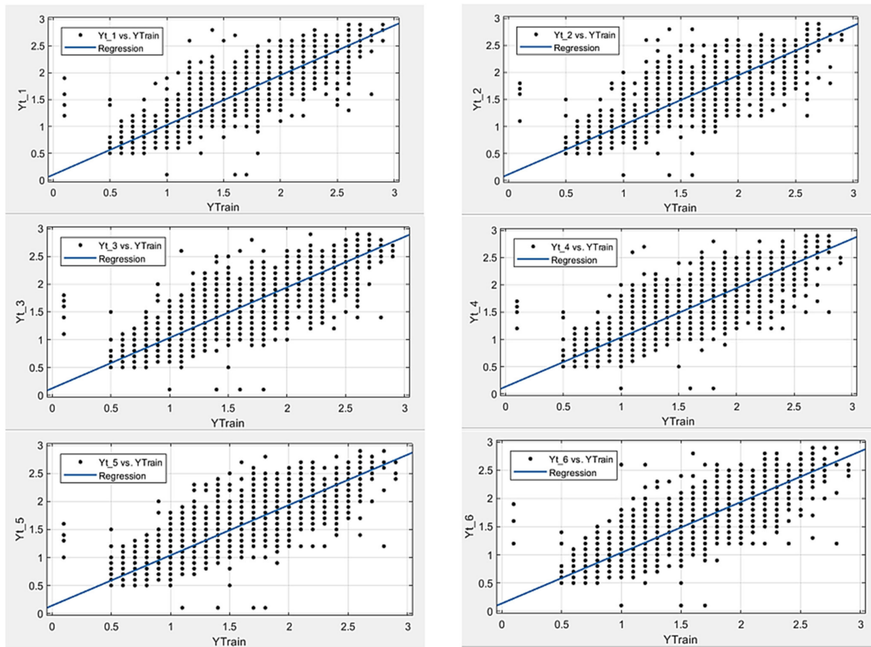
Figure 6. Correlation with the previous six load lags.
