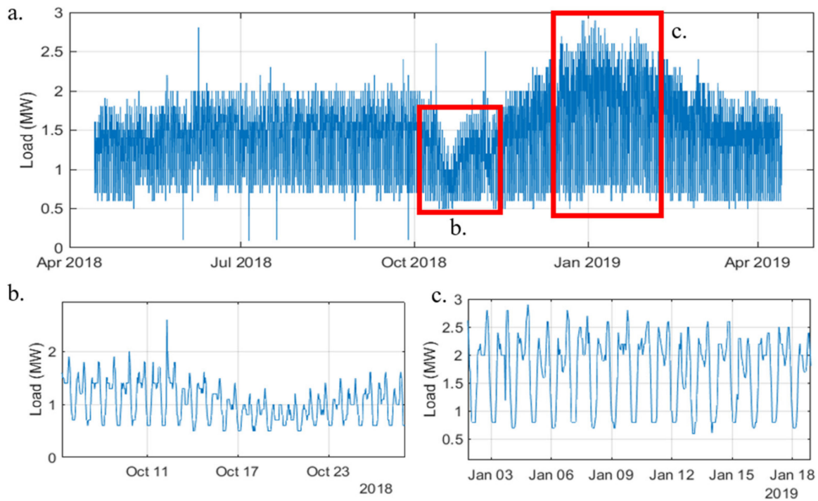
Figure 1. (a) One year of hourly load demand at a Baneshwor substation (from April 2018 to April 2019). (b) Zoomed in section of electricity consumption in October (lower consumption). (c) Zoomed in section of electricity consumption in January (high consumption).
