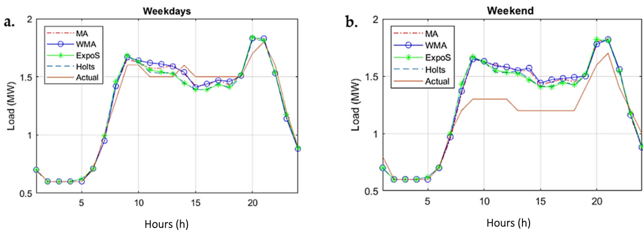
Figure 10. Actual vs. predicted forecasts achieved by conventional time series models. (a) Weekday forecasting. (b) Weekend forecasting.
