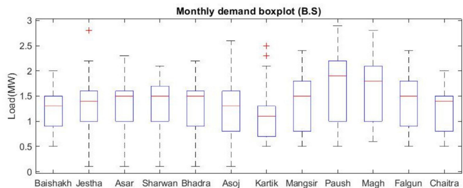
Figure 2. Boxplot of electricity demand for each month (B.S.).
