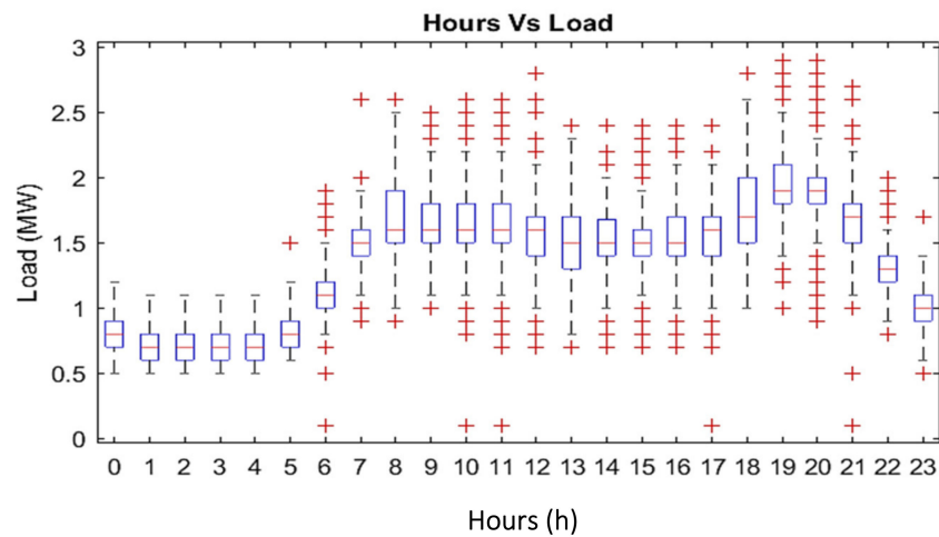
Figure 4. Box plot of electricity demand for each hour.
