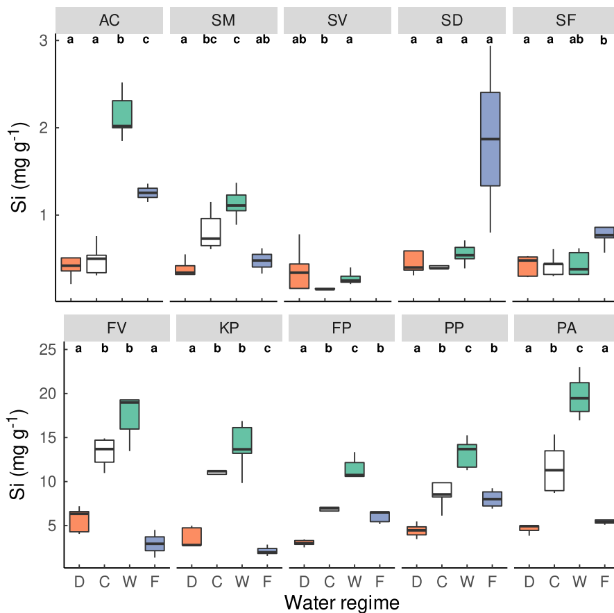
FIGURE 2 Plant Si concentrations of forbs (upper panel) and grasses (lower panel; five species each) under four water regimes (D = drought; C = control, i.e. benign conditions; W = waterlogging; F = flooding). Box plots show medians, 25th and 75th percentiles (interquartile range), and 1.5 \times interquartile ranges without outliers. Results of Tukey post-hoc tests conducted within each species are given as letters with each letter indicating groups which did not differ significantly. See Table 2 and Table S1 for details and Table 1 for species abbreviations.
