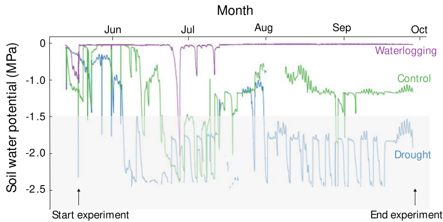
FIGURE 1 Soil water potentials during the mesocosm experiment in the drought, control and waterlogged treatment. Black arrows indicate start and end of the experiment and coloured lines represent different water regimes. No measurements were taken in the flooded treatments as water potentials in the fully submerged soil were assumed to be 0 MPa. The gypsum blocks used to monitor water potentials have a measurement range down to -1.5 MPa. Lower readings (grey area) therefore indicate water potentials below -1.5 MPa (considered the permanent wilting point) but do not represent the actual water potentials. For visualization values were aggregated into hourly values. See methods for details.
