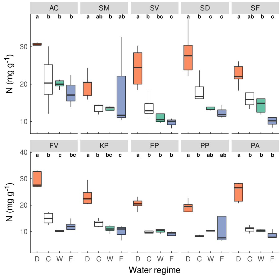
FIGURE 3 Plant N concentrations of forbs (upper panel) and grasses (lower panel; five species each) under four water regimes (D = drought; C = control, i.e. benign conditions; W = waterlogging; F = flooding). Box plots show medians, 25th and 75th percentiles (interquartile range), and 1.5× interquartile ranges without outliers. Results of Tukey post-hoc tests conducted within each species are given as letters with each letter indicating groups which did not differ significantly. See Table 2 and Table S1 for details and Table 1 for species abbreviations.
