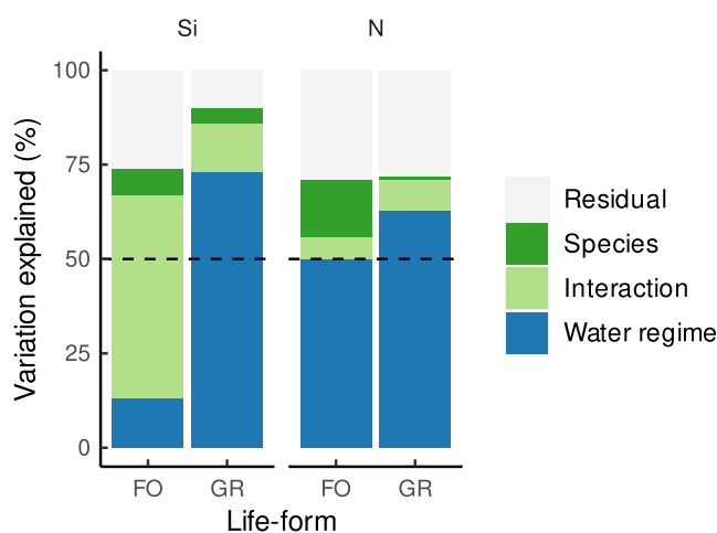
FIGURE 5 Partitioning of the observed total variation of plant Si and N concentrations in five grass and five forb species under four water regimes ranging from dry to flooded conditions. Colours indicate the amount of variation explained by plasticity in response to water regimes (dark blue) and species-specific responses (interaction, light green), as well as species differences (dark green) and residual variation not explained by any of these factors (grey). Values were derived from variance estimates of random factors of random intercept models. For details see Section 2.
