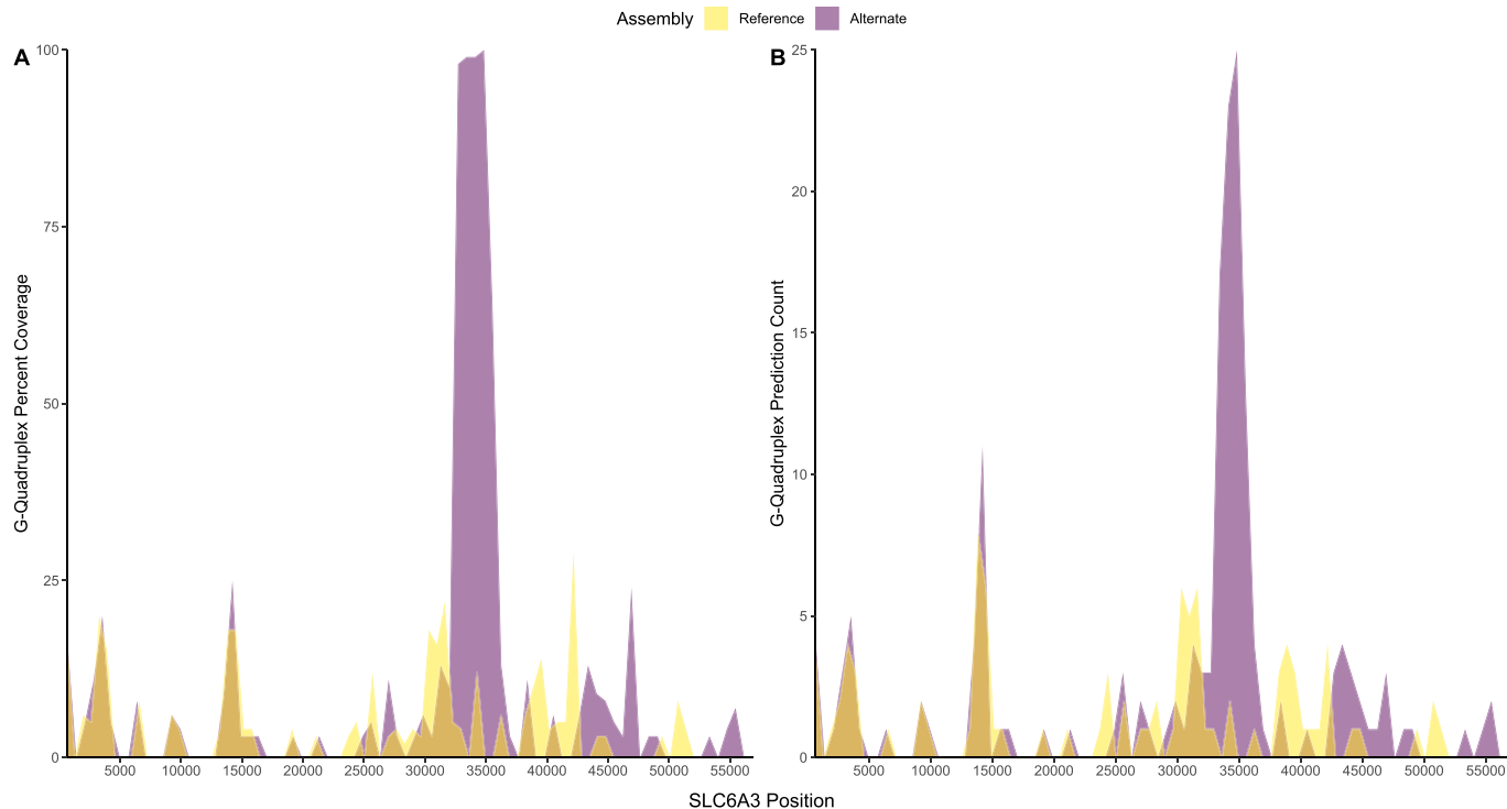
Figure 5. G4-Hunter results for SLC6A3 sequences from the human reference genome (GRCh38/hg38; yellow) and the alternate human reference genome (KI270791v1; purple). (A) shows the G4 coverage percentage in each section of SLC6A3 . (B) shows the G4 count in each section of SLC6A3 .
