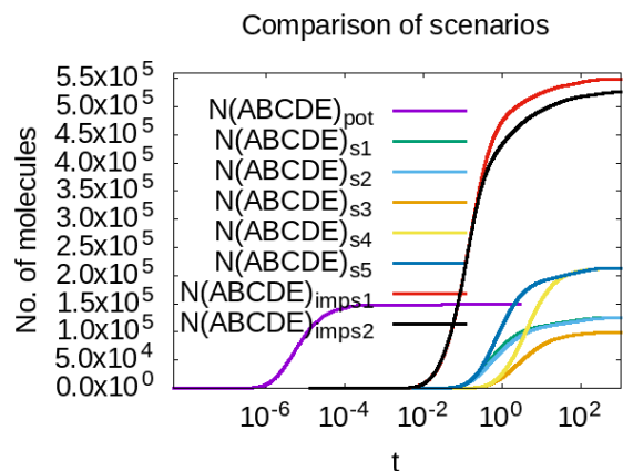
Figure 5: Simulation results for the one-pot reaction (pot), scenarios (s1) to (s5) and the scenarios improved by the compiler, (imps1) and (imps2). The latter produce a much higher yield compared to any other scenario, and, with the exception of the one-pot reaction, are also faster.
