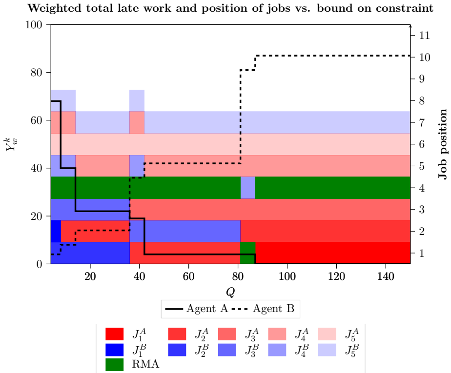
Figure 1. Solving 1 | \text{RMA} | Y_w^A : Y_w^B \leq Q for different values of Q with T = 10 and data from Table 2
