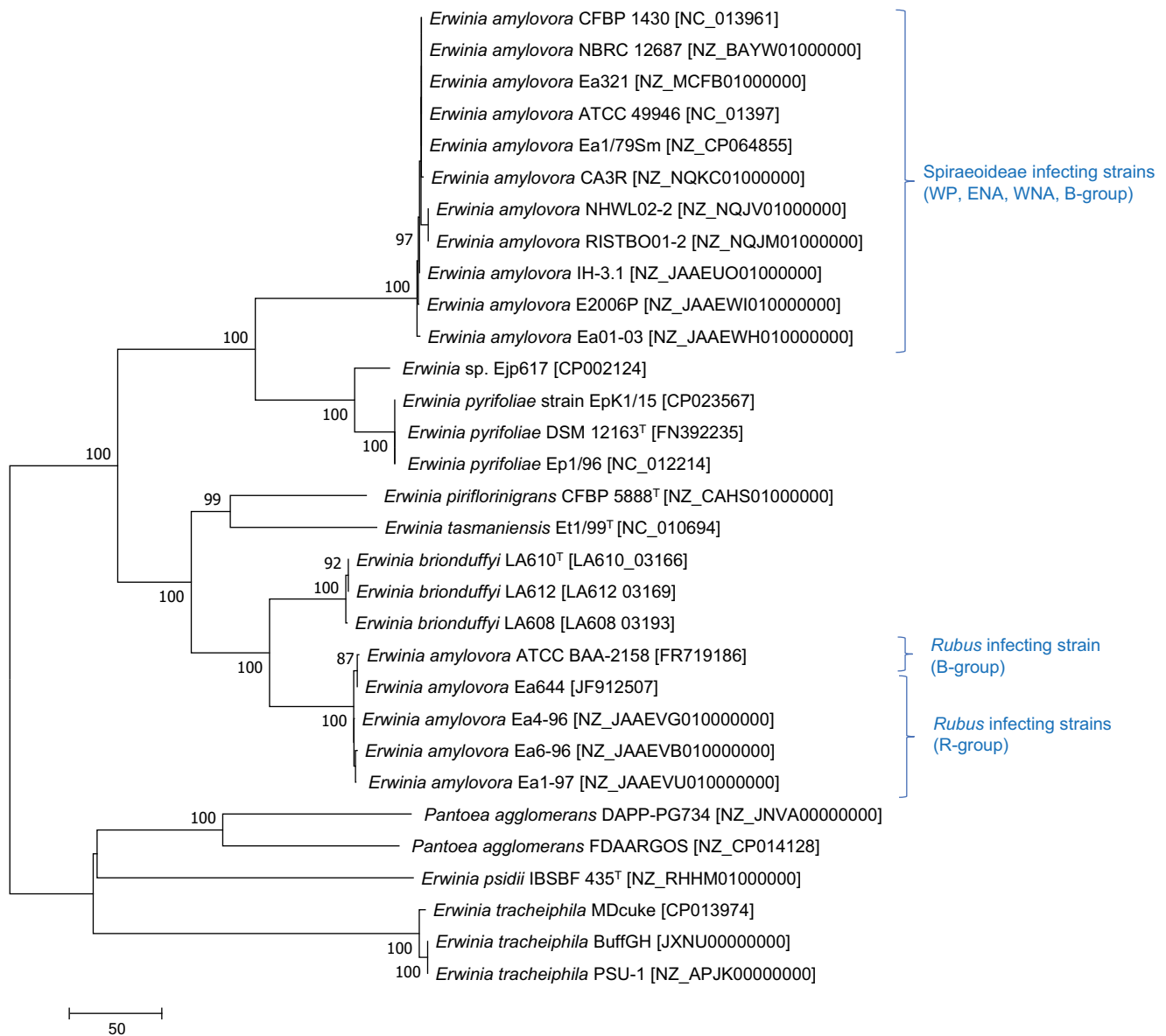
Fig. 2 Phylogenetic analyses of the type III secretion system gene eopI from strains of different species within the genus Erwinia . Rubus -infecting isolates cluster separately from their Amygdaloideae-infecting counterparts suggesting convergent evolution of some strains
