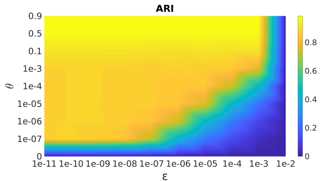
Fig. 3. Sensitivity of \varepsilon and \theta with respect to the ARI measure.
