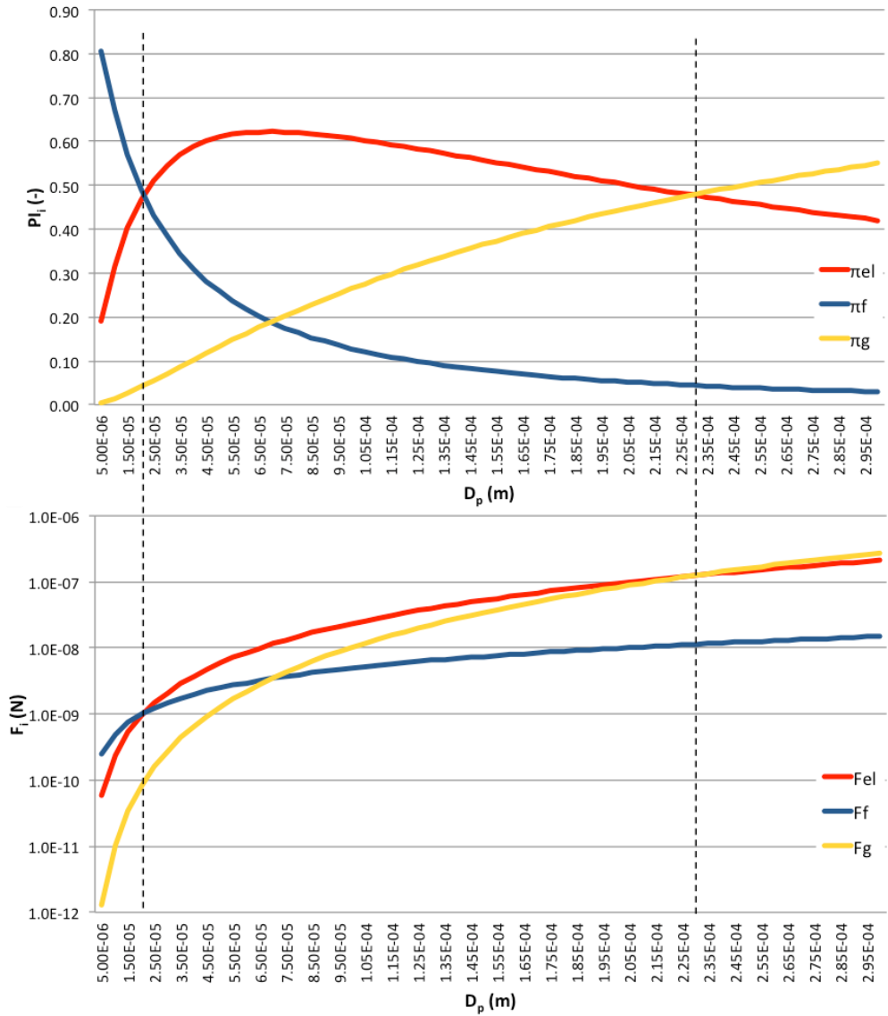
Figure 2: Exemplary case ( \rho_p = 1300\text{kg/m}^3 , q_p = 1\text{C/m}^2 , \max(v_{p,a}) = 0.1\text{m/s} , \max(E) = 0.75\text{ N/C} , \mu_a = 1.98\text{e-}5\text{ Pas} ) of maximum acting particle forces (bottom) and dimensionless force groups \pi_i (top) against particle diameter D_p . D_p < 20\mu\text{m} : dominance of fluid drag force; 20\mu\text{m} < D_p < 230\mu\text{m} : dominance of electric forces; D_p > 230\mu\text{m} : dominance of gravity force.
